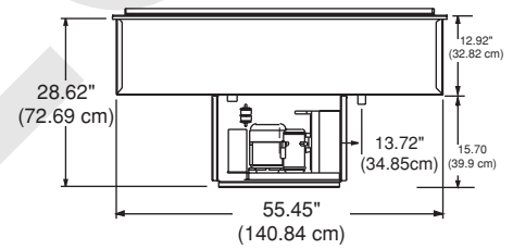
ELEVATION VIEW N8157-FA
